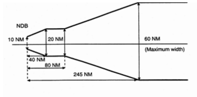
Figure 2: Corridor width from an NDB
