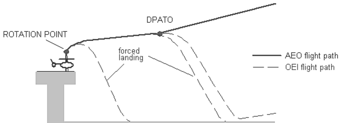
Figure 1: Take-off profile
