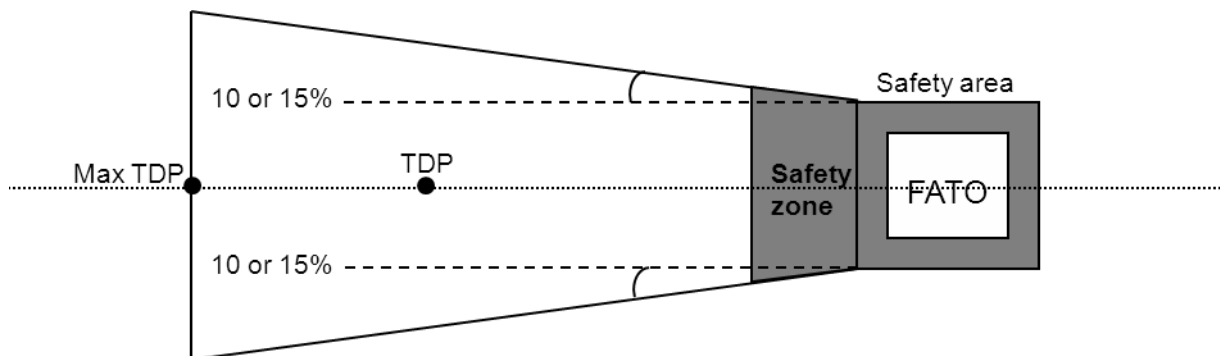
Figure 2: Obstacle accountability
